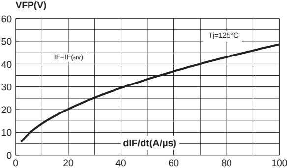
Fig. 8: Transient peak forward voltage versus dI_F/dt .
